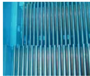
Vibrating grizzly bars For the pre-screening at small apertures of sticky material, generally located on the lower deck
