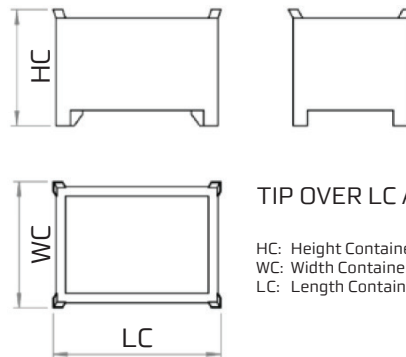
CONTAINER SIZE
