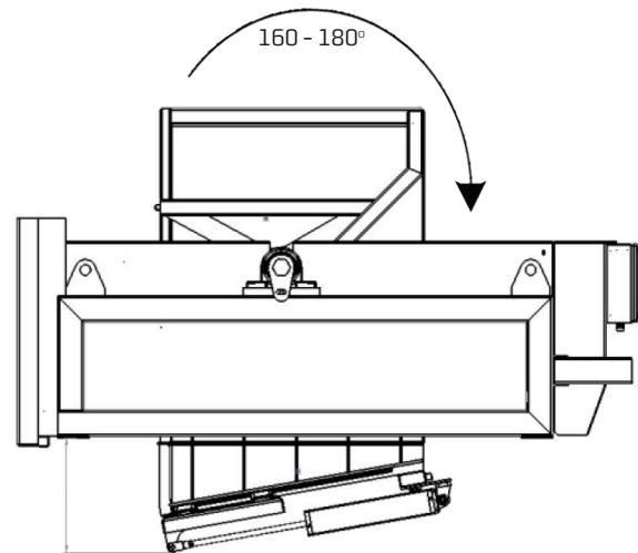
UNLOADING POSITION
