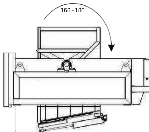
POSITION DECHARGEMENT
