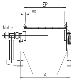
PULLY/BELT SYSTEM
