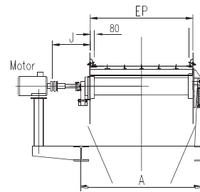
DIRECT DRIVE
